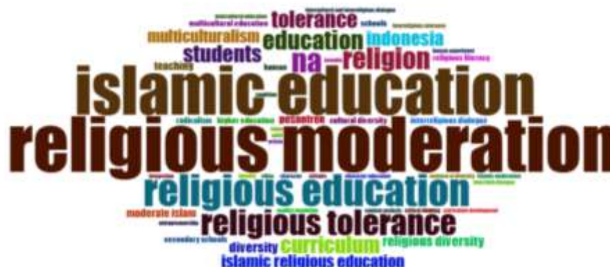
Gambar 8. Word Cloud
