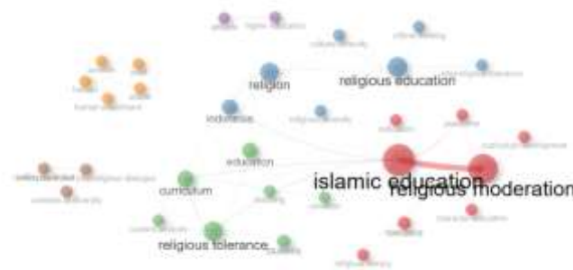
Gambar 10. Jaringan Co-Occurrence
